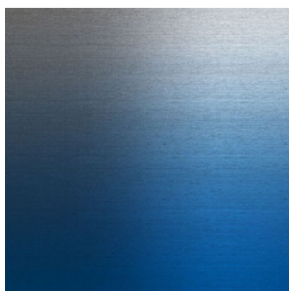
COBALT
