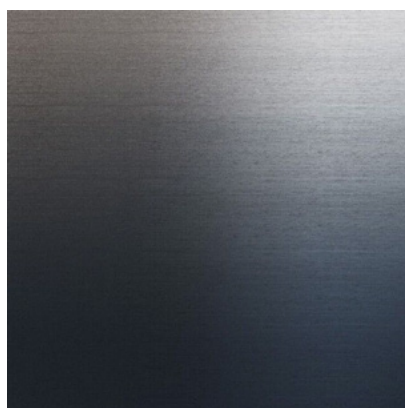
SHALE
