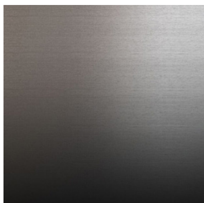
OBSIDIAN
